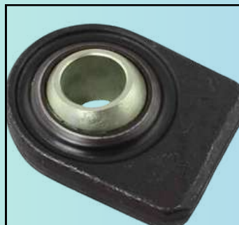
ZIRCON BOTTOM LINK BALL END WELD ON CATII 28.5X80 FS1342 (YSM 10)
